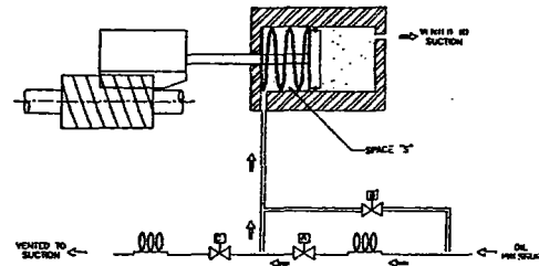
FIGURE 2-8: UNLOADING
